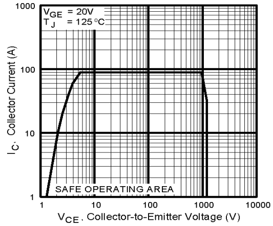
Fig. 12 - Turn-Off SOA
